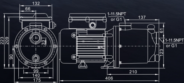
Overall dimension
