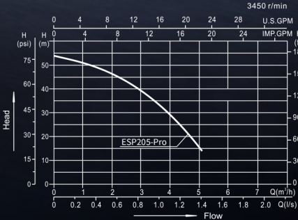
Performance curves
